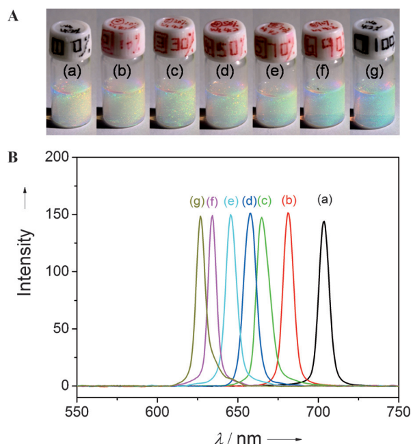
Figure 1. A) Photographs of colloid crystals assembled from PNIPAM microgel dispersions containing 0% (a), 10% (b), 30% (c), 50% (d), 70% (e), 90% (f), and 100% (g) P(NIPAM-AAc) microgel. B) Reflection spectra of the microgel colloidal crystals. The pH value of the dispersions is about 3.5. The hydrodynamic radius at 20 °C and pH 3.5 is 160 nm for PNIPAM and 158 nm for P(NIPAM-AAc), respectively.
